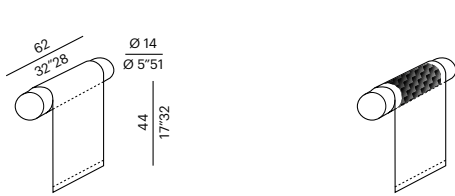
poggiatesta rullo - headrest roll
