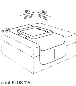
vassoio tasca - tray/pocket C-C2
