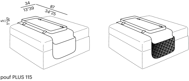
vassoio tasca - tray/pocket B-B
